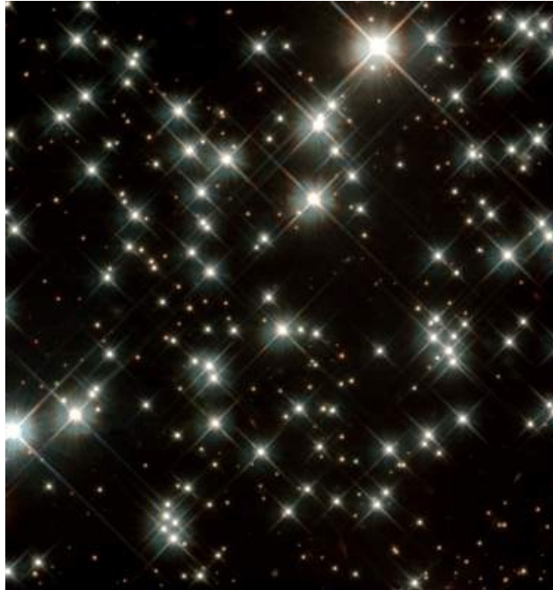
Figure 1. White dwarfs in the globular cluster M4. In this picture, only the faintest stars are white dwarfs. © NASA and H. Richer (University of British Columbia)
